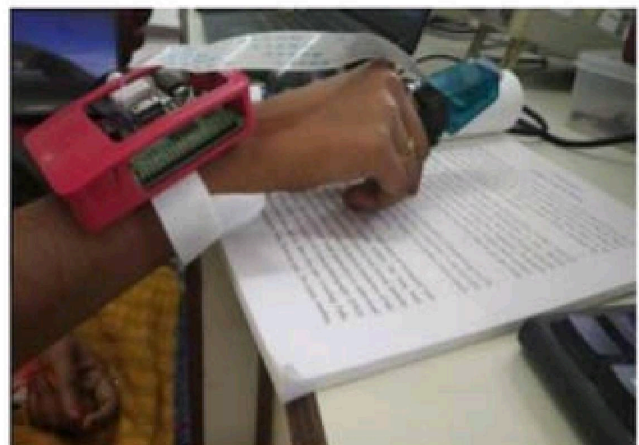
Fig. 5.27 Wearable reader
